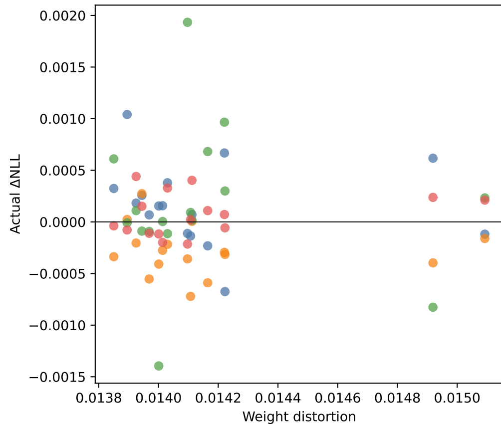
Figure 5: Distortion/risk proxy vs actual \Delta NLL (4-bit)
