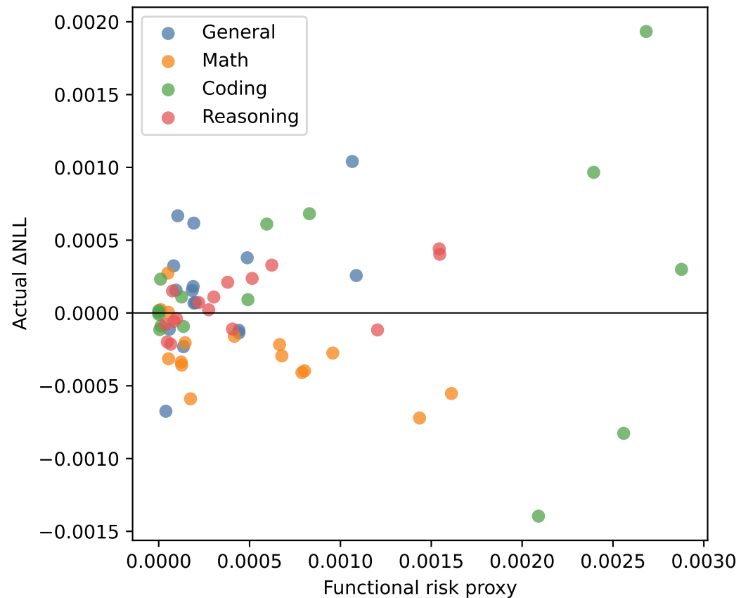
Figure 5: Distortion/risk proxy vs actual \Delta NLL (4-bit)
