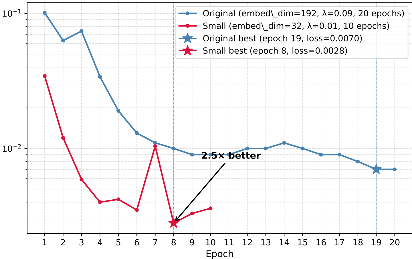
Validation Prediction Loss (log scale)
