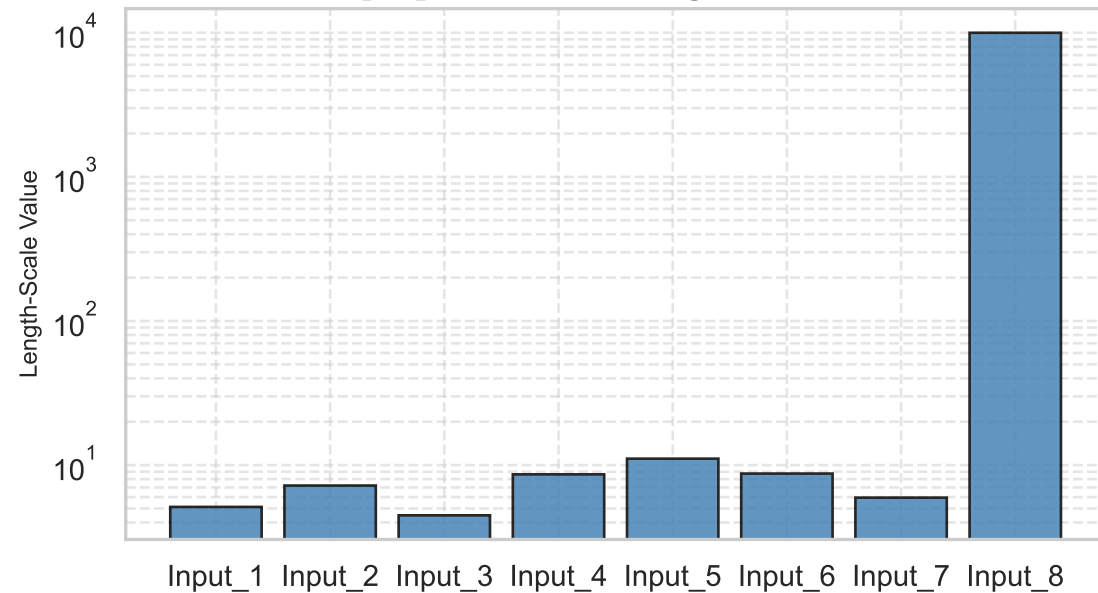
[F8] GPR RBF Length-Scales
