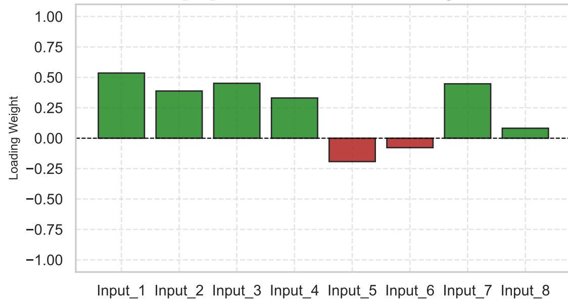
[F8] PCA PC1 Feature Loadings
