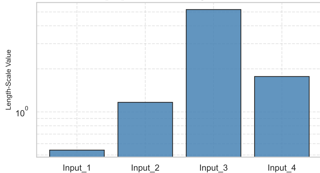
[F4] GPR RBF Length-Scales
