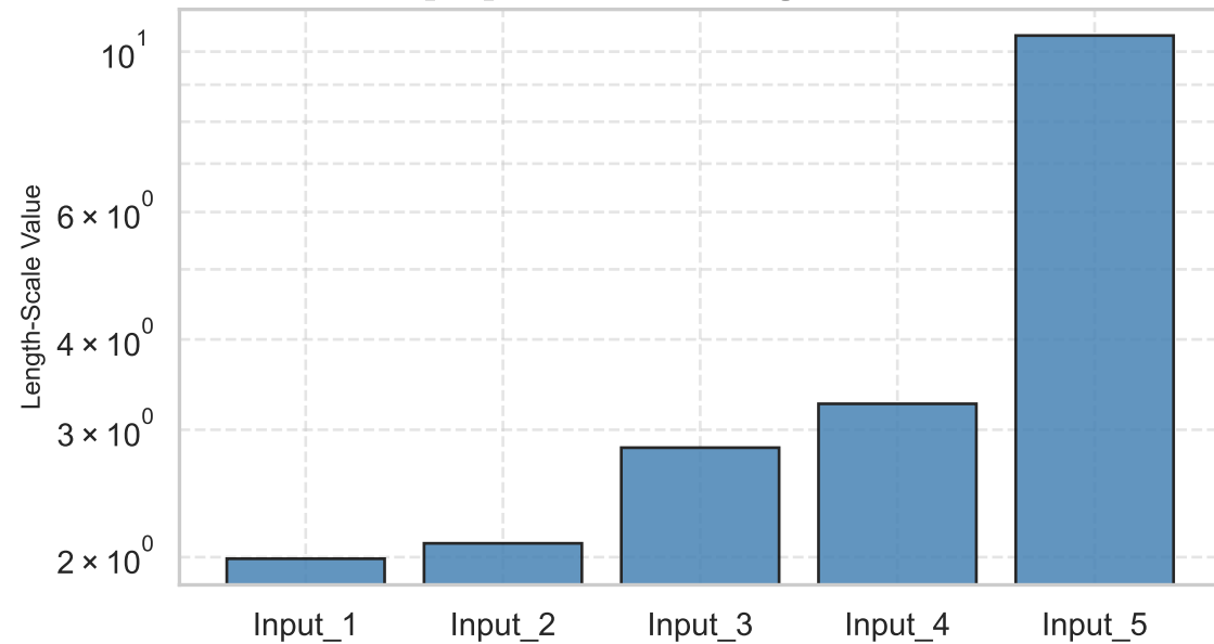
[F6] GPR RBF Length-Scales
