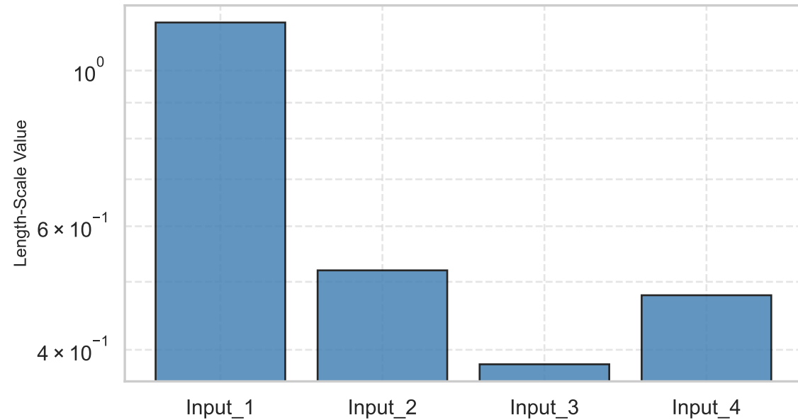
[F5] GPR RBF Length-Scales
