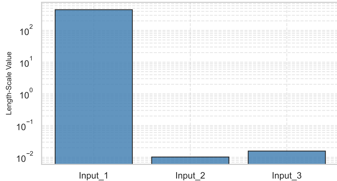
[F3] GPR RBF Length-Scales
