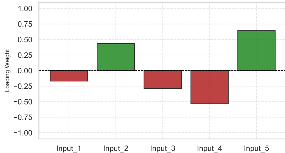
[F6] PCA PC1 Feature Loadings
