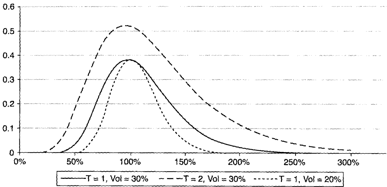
Figure 5.8 Effects of different volatilities and maturities on a European's Vega.
