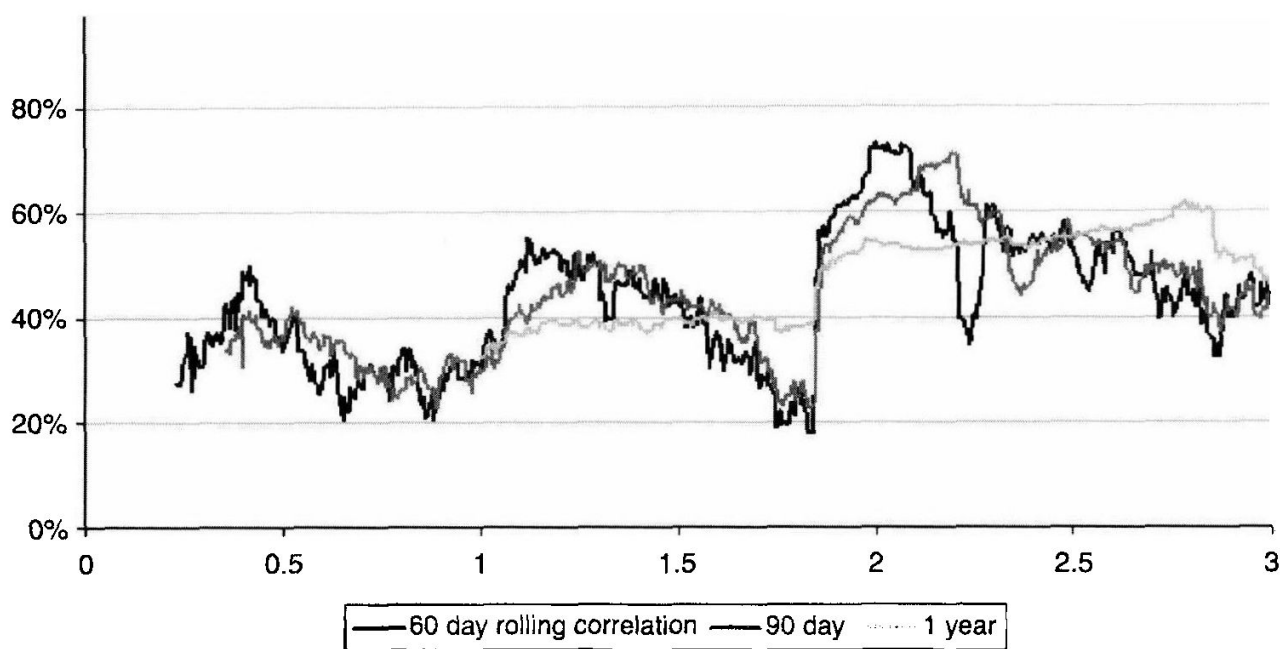
Figure 7.2 The time series of the 60-day, the 90-day and the 1-year rolling correlation. The correlation is computed based on the daily price of the two underlyings in Figure 7.1.
