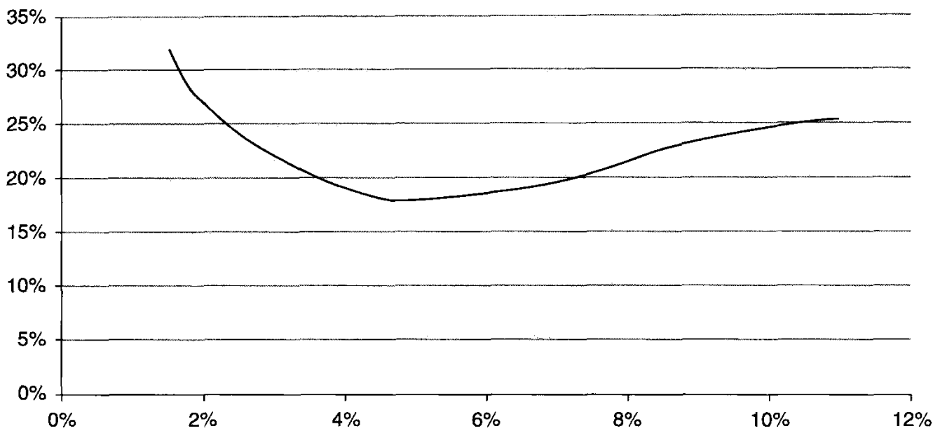
Figure 17.2 The implied volatility smile of a European swaption. Deep OTM call option implied volatilities tend to flatten out the deeper one goes OTM. The smile shape is different to the equity skews.
