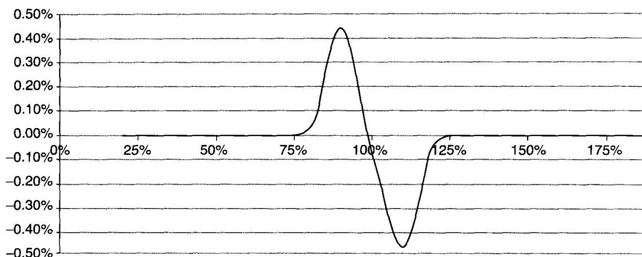
Figure 11.4 The Gamma of a call spread.
