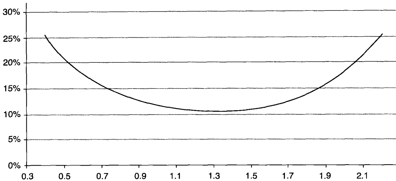
Figure 18.2 An example of an implied volatility smile for the EUR–USD. The smile is (almost) symmetric.
