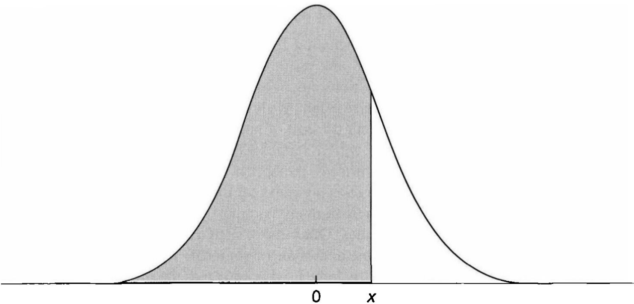
Figure 3.6 The cumulative probability distribution function for a standardized Normal distribution. Note that the shaded area represents \mathcal{N}(x) which is the probability that a normally distributed variable with mean 0 and variance 1 will be lower than the value x . Because of the symmetry of the standard Normal distribution, one can easily figure out that \mathcal{N}(-x) is represented by the non-graded area. Note that the area under the bell curve is equal to 1.
