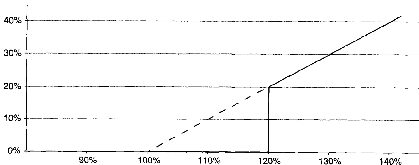
Figure 10.8 Payoff of an up-and-in ATM call option with knock-in barrier at 120%.
