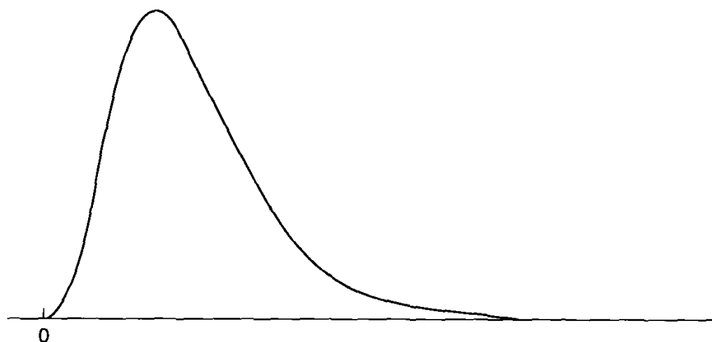
Figure 3.4 A log-normal distribution.
