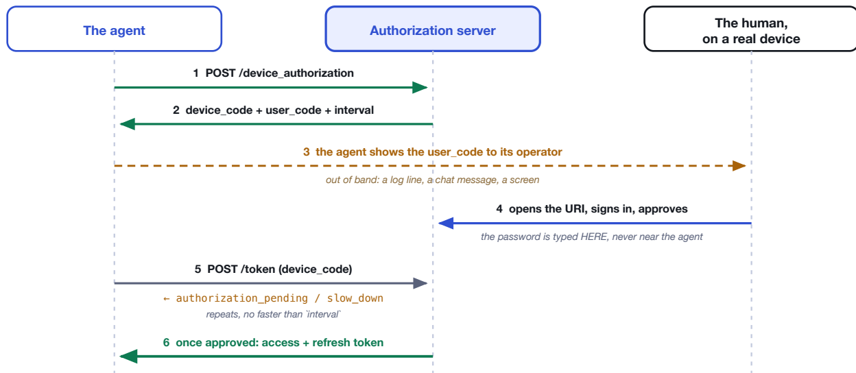
Figure 14.2 — The agent never handles a credential and never needs a redirect URI. The only thing it shows the operator is a short code that is useless to anyone who cannot also authenticate.
