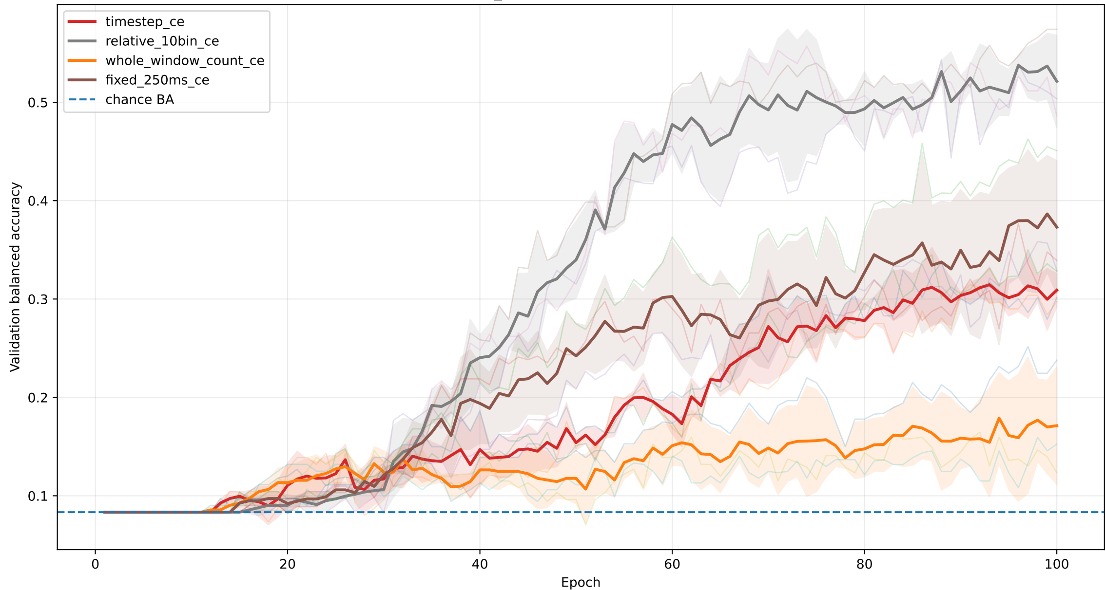
Experiment 2.1.2 — Validation BA vs epoch single hidden shift_syn=2, mean \pm SD across paired seeds
