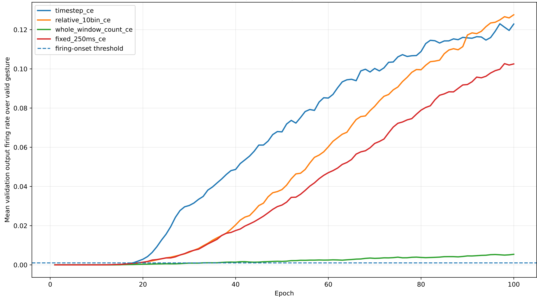
How each objective escapes the silent regime
