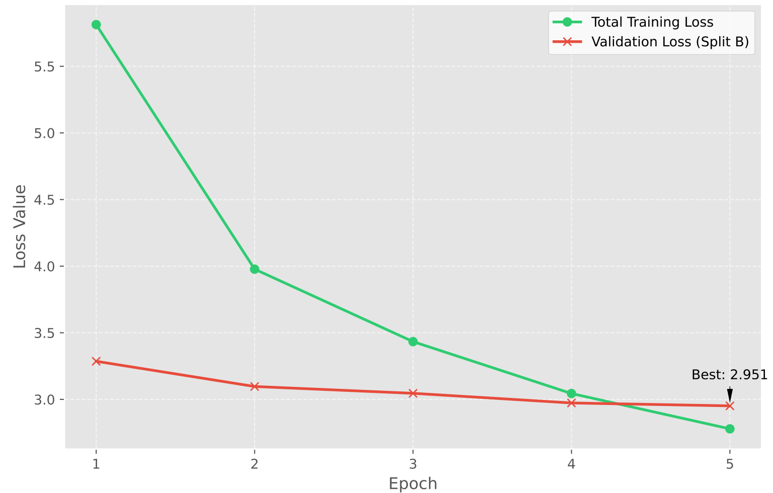
Model Generalization (Train vs. Val)
