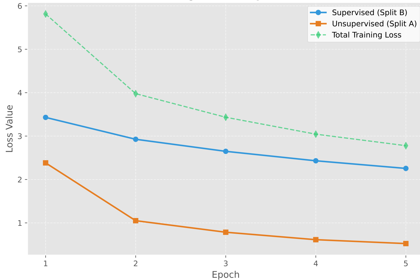
Training Loss Components
