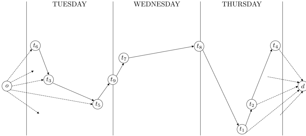
Figure 4.1: Example of a graph D where only the path corresponding to the block of Figure 3.3 is made explicit (the last duty in this block being the one of Figure 3.2). Let P_1 := o, t_6, t_3, t_5, t_9, t_7, t_8, t_1 be the path from o to t_1 using the arcs explicited in the graph. The 1st component of r_{P_1} measuring the number of working days in the current partial block is 4. The 6th component of r_{P_1} , measuring the work range in the current partial duty (covering train t_1 ), is 1h53. The 7th component of r_{P_1} , measuring the work range in the duty just completed (covering train t_8 ), is 8h13. Let P_2 be the path obtained from P_1 by adding the arc from t_1 to t_2 . The 1st component of r_{P_2} is 4. The 6th and 7th components of r_{P_2} , which consider the duty covering trains t_1 and t_2 , have the same value equal to 2h12. Let P_3 be the path obtained from P_2 by adding the arc from t_2 to t_4 . The 1st component of r_{P_3} is 4. The 6th and 7th components of r_{P_3} , which consider the duty covering trains t_1 , t_2 , and t_4 , have the same value equal to 8h04. Let P_4 be the path obtained from P_3 by adding the arc from t_4 to d . The 1st component of r_{P_4} is 5 (according to rule R20, the last duty must be followed by an on-call, counted when the path is completed). The 6th and 7th components of r_{P_4} have the same value equal to 8h17.
