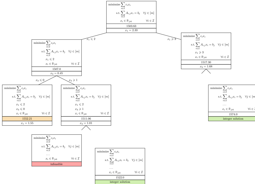
Figure A.1: An illustration of the branch-and-price algorithm: the right side of the tree is explored first and the best integer solution is updated with value 1574.0. Then the left nodes are explored. The node with value 1552.21 does not generate children nodes as its value is worse than the best integer value. Then the infeasible node does not generate any children nodes either. The next best integer solution has value 1522.0. When all nodes have been explored, we have found the optimal integer solution.
