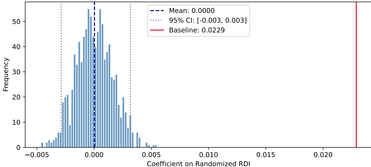
Placebo Distribution: Randomized RDI Within Year
