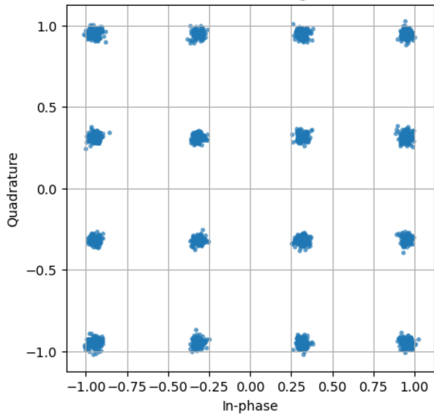
16QAM Constellation @ 30.0 dB
