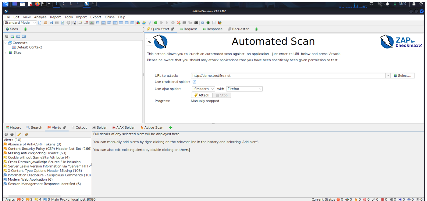
Figure 2: OWASP ZAP alert showing vulnerability
