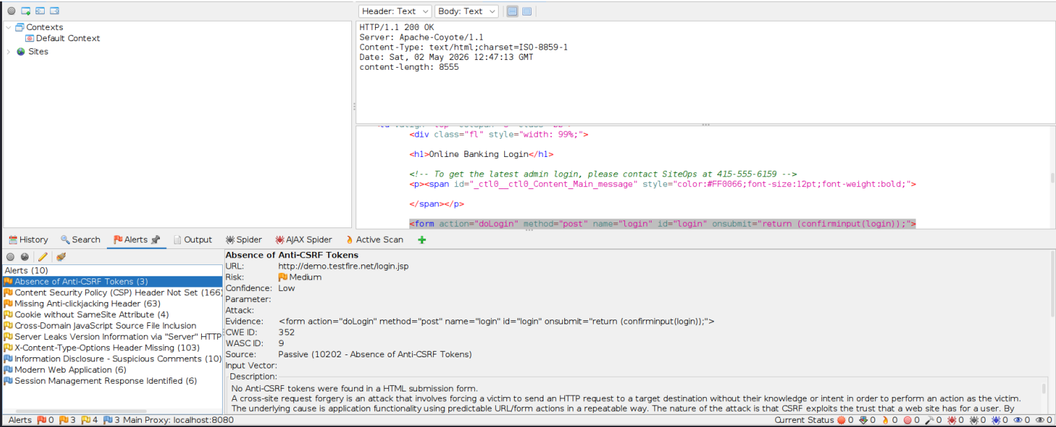
Figure 3: OWASP ZAP alert showing absence of Anti-CSRF protection
