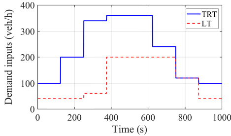
Fig. 5. Demand inputs for each turning direction at the origins O_1 to O_6 .
