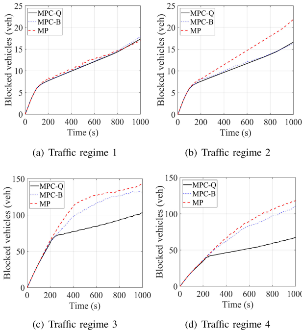
Fig. 12. Evolution of blocked vehicles A_q for varied demand profiles with different methods.
