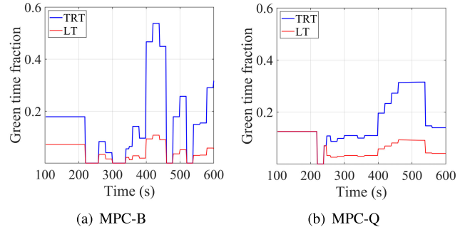
Fig. 8. Comparison of control stability in terms of effective fraction of green time for road segment 1 associated with MPC-B and MPC-Q.
