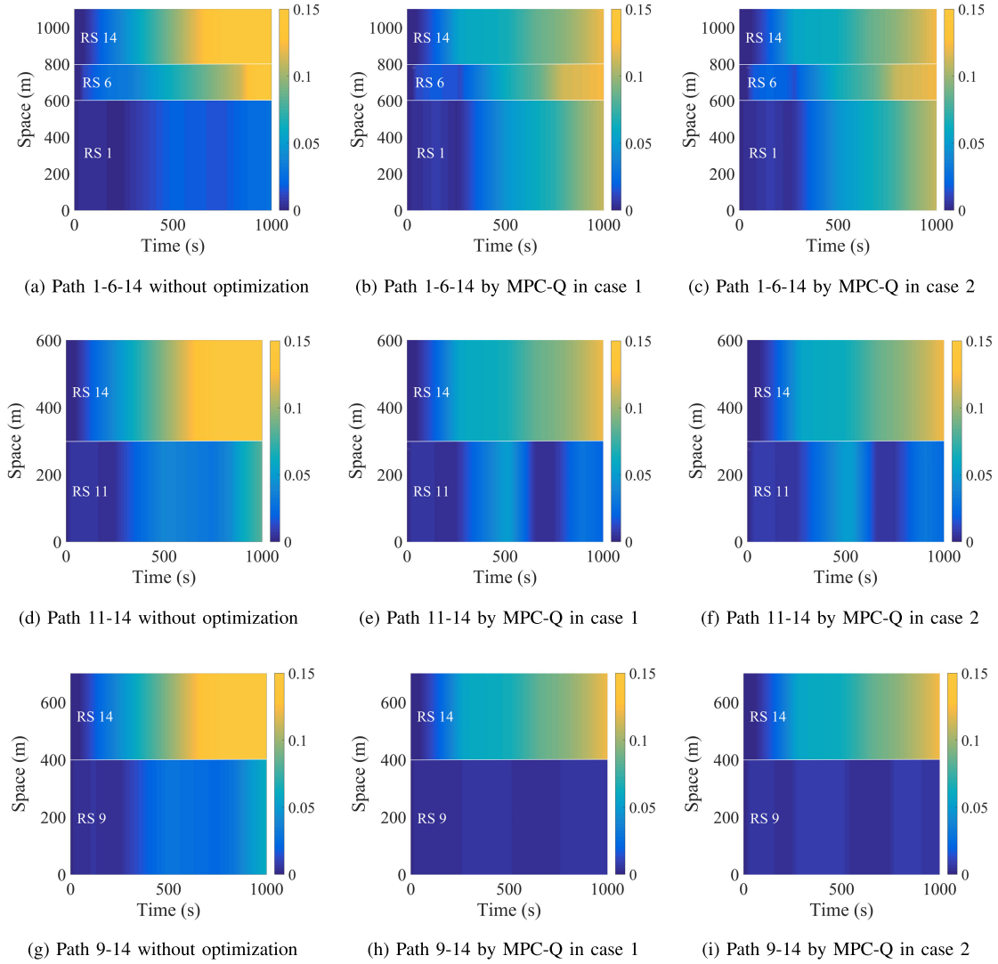
Fig. 10. Evolution of space-time average density (veh/m) on bottleneck-related paths by MPC-Q with model errors.
