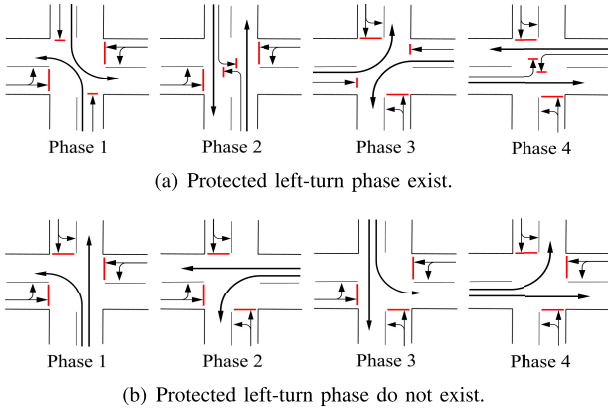
Fig. 3. Illustration of signal phases at the local intersection.
