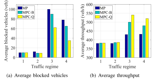
Fig. 13. Comparison of average blocked vehicles and throughput under different traffic regimes using different control methods.
