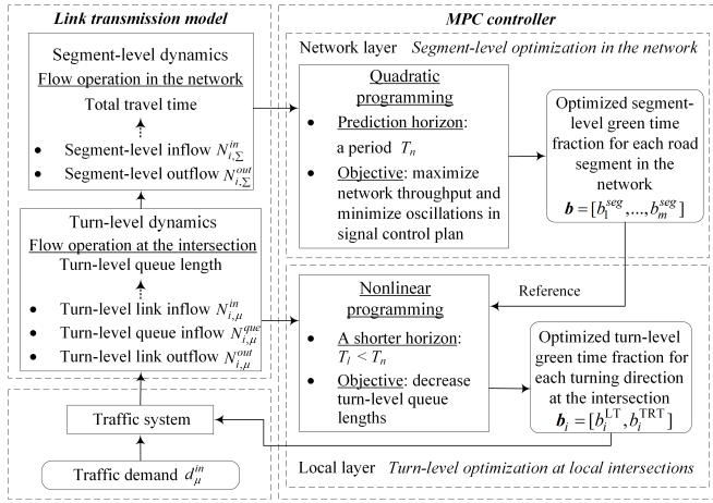
Fig. 1. Hierarchical framework of the proposed MPC-Q. \mathbf{b} = [b_1^{seg}, \dots, b_m^{seg}] is the set of segment-level effective fractions of green time for all m road segments in the network; \mathbf{b}_i = [b_i^{LT}, b_i^{TRT}] is the set of turn-level effective fractions of green time for left-turn (LT) and through/right-turn (TRT) directions of road segment i , respectively. Note that the time index k is omitted from notations, but all the variables are time-dependent.
