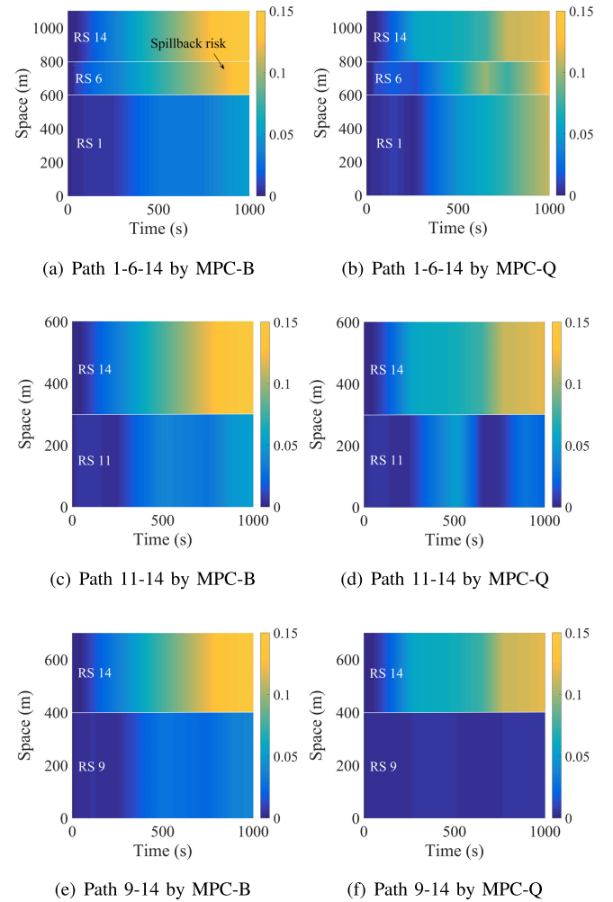
Fig. 6. Evolution of space-time average density (veh/m) on bottleneck-related paths using MPC-B and MPC-Q.
