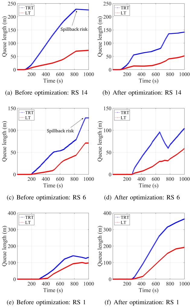
Fig. 7. Comparison of turn-level queue length changes at Path 1-6-14 before and after the optimization, where RS represents road segment.
