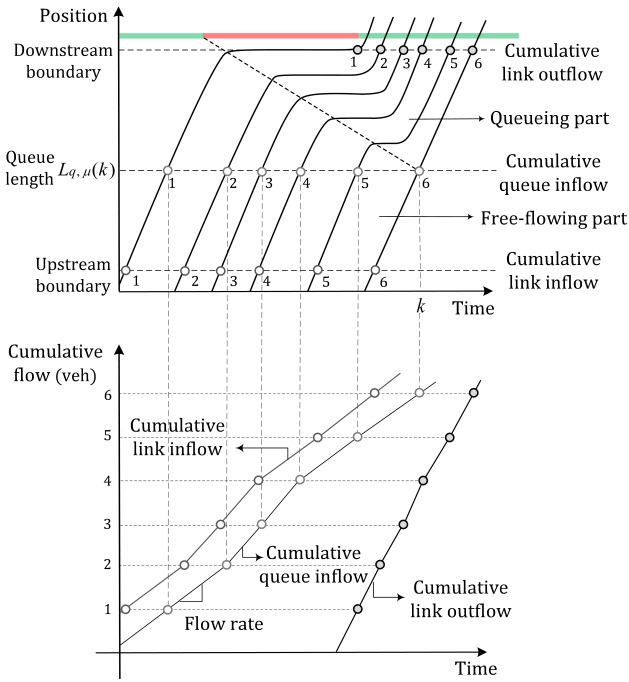
Fig. 2. Illustration of flow dynamics determined by the LTM with queue transmission. An road segment with length L_i is, for each in turning direction \mu , divided into the free-flow and queueing parts of lengths L_{f,\mu}(k) and L_{q,\mu}(k) , respectively.
