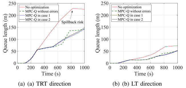
Fig. 9. Comparison results of queue length at bottleneck link 14 under model errors.
