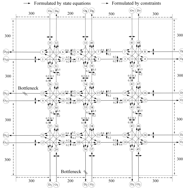
Fig. 11. Illustration of the simulated grid network.
