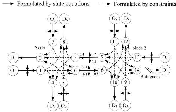
Fig. 4. Illustration of the arterial with successive intersections, where O_1 to O_6 represent the origins; D_1 to D_6 represent the destinations; the bottleneck is located on road segment 14; the paths related to the bottleneck are 1-6-14, 9-14, and 11-14.
