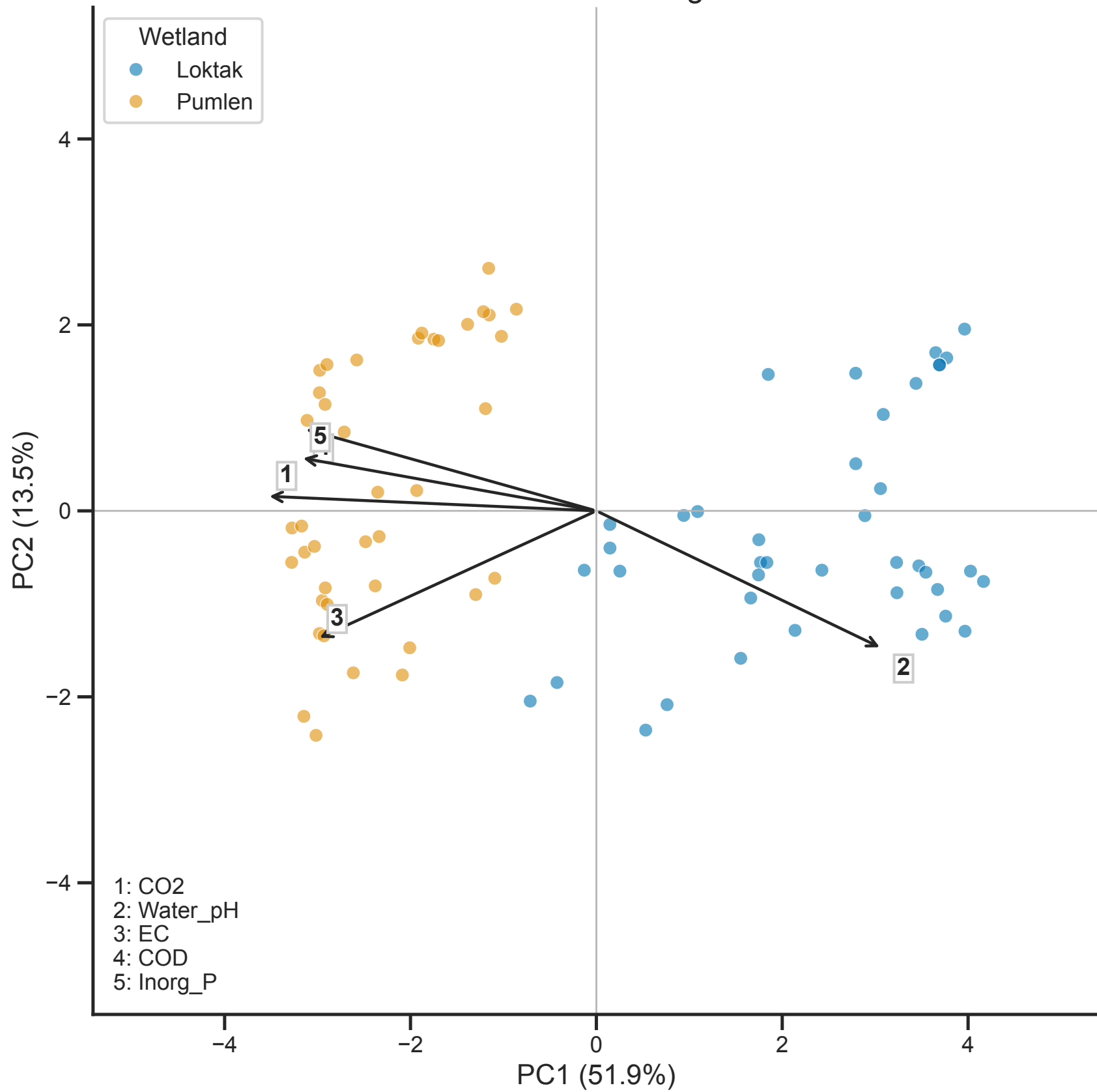
Water: scores + loadings × 3.79
