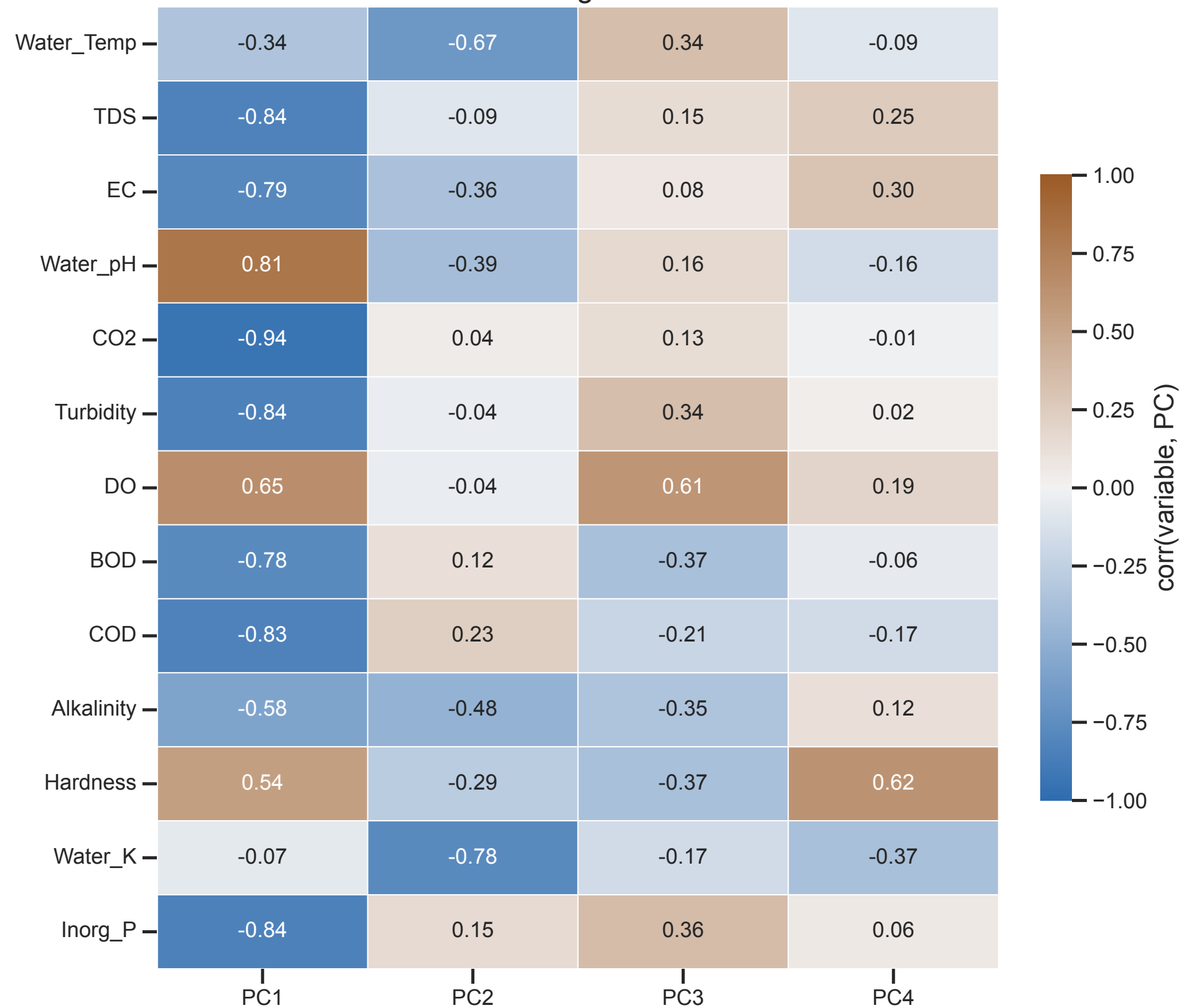
Correlation loadings — all variables
