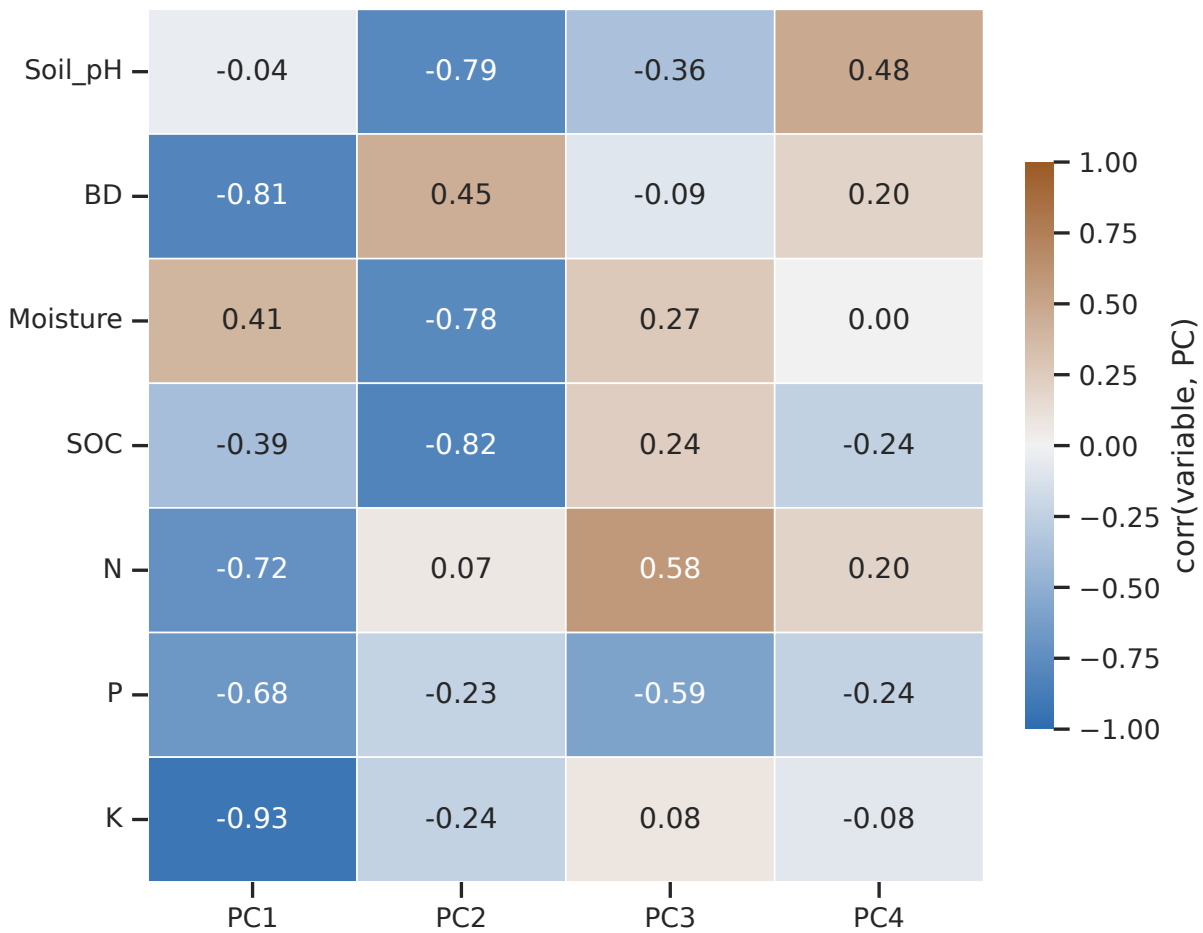
Soil PCA: correlation loadings
