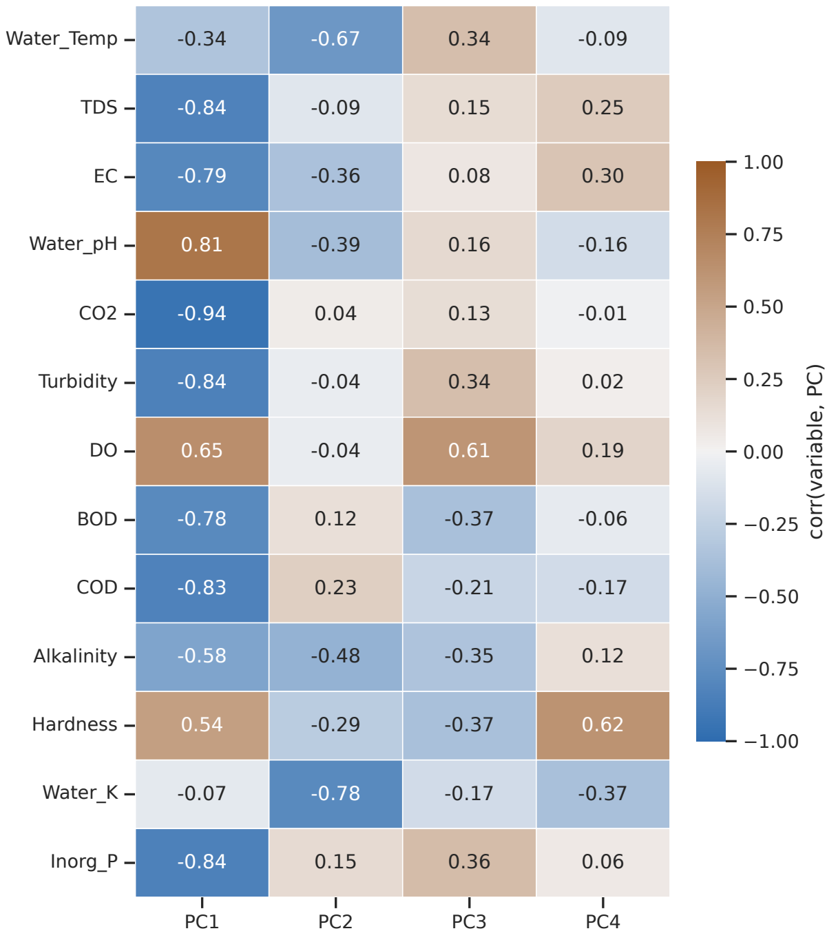
Water PCA: correlation loadings
