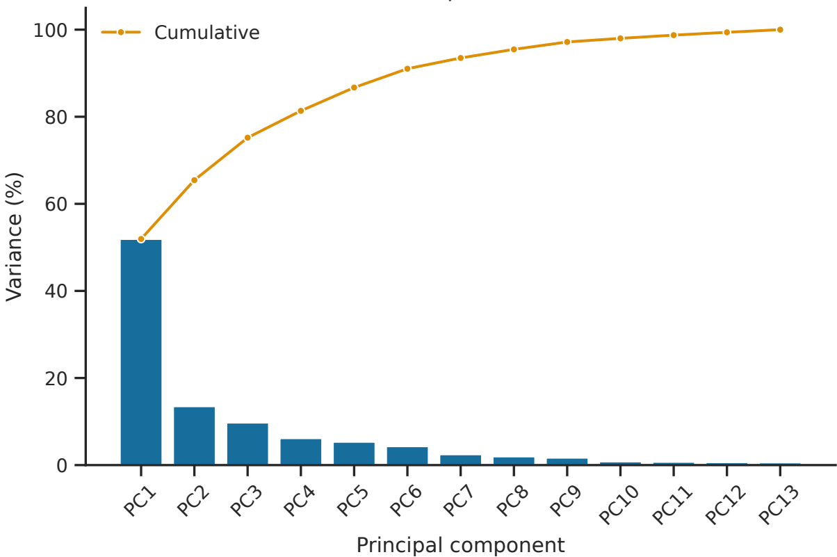
Water PCA: explained variance
