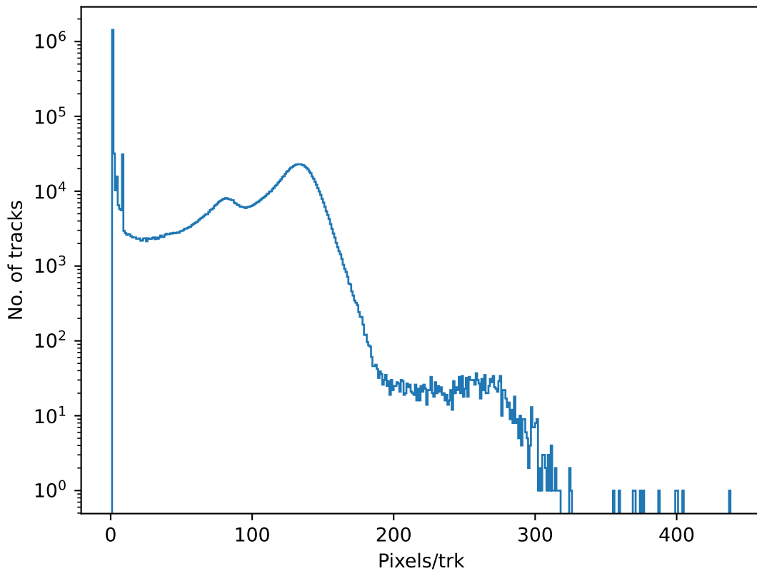
Trk Size (nrow) hist Ct rate : 14850.51 sec-1
