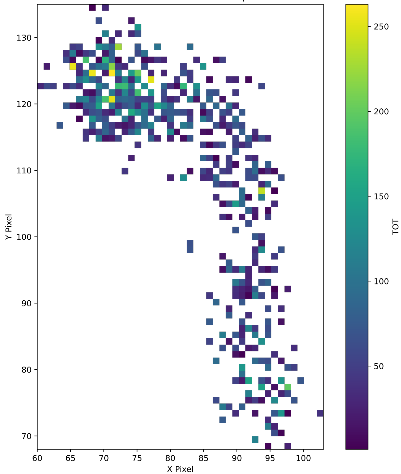
TrkID-193721 TOT Pixel Map
