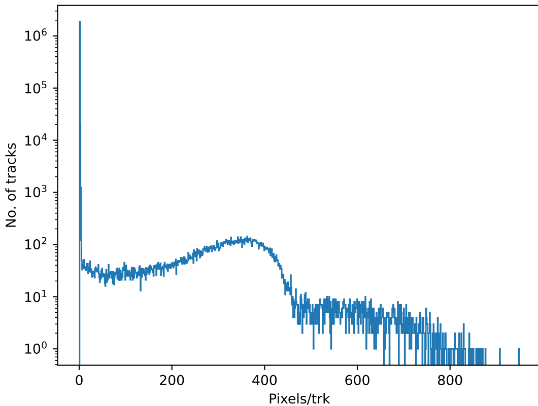
Trk Size (nrow) hist Ct rate : 1064.38 sec-1
