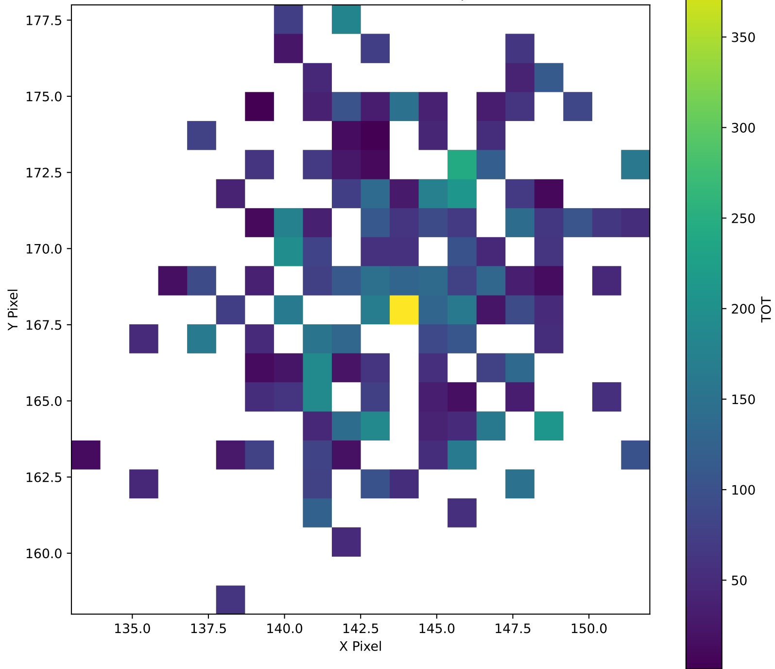
TrkID-120506 TOT Pixel Map
