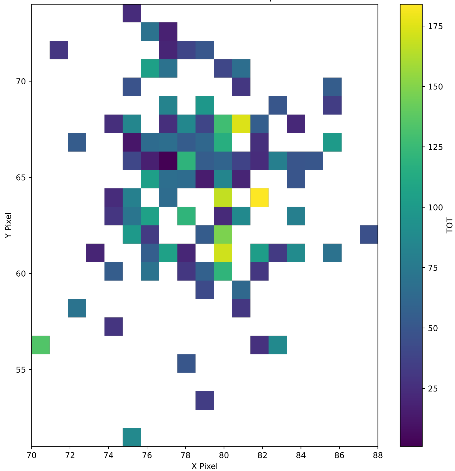
TrkID-1246927 TOT Pixel Map
