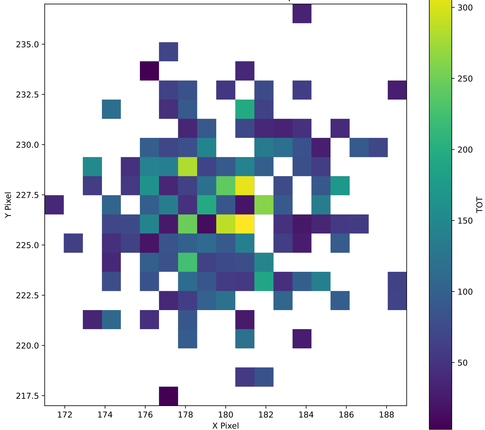
TrkID-126968 TOT Pixel Map
