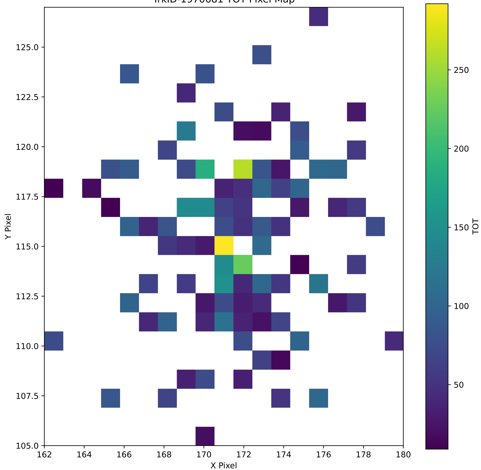
TrkID-1970681 TOT Pixel Map
