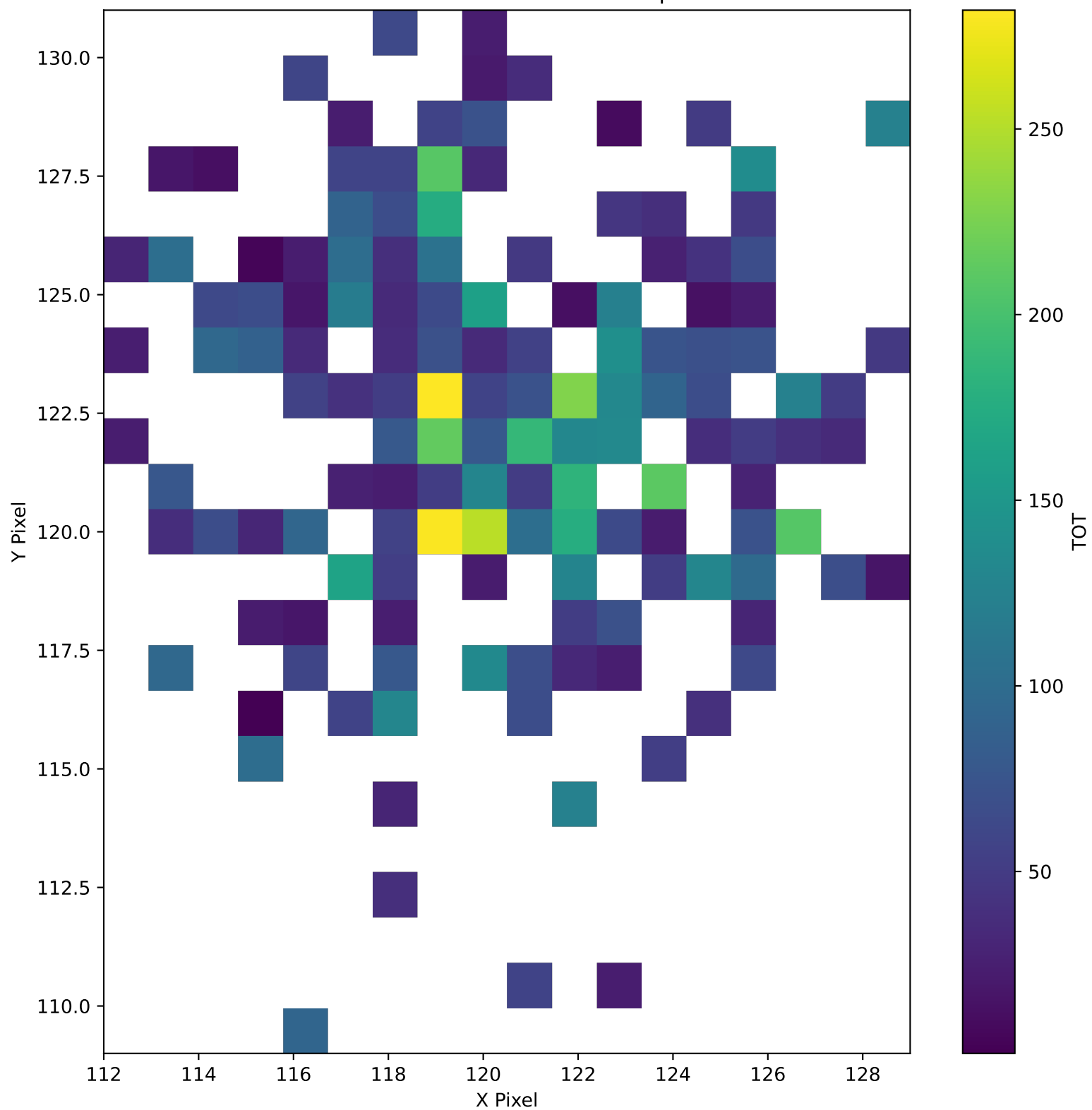
TrkID-1929604 TOT Pixel Map
