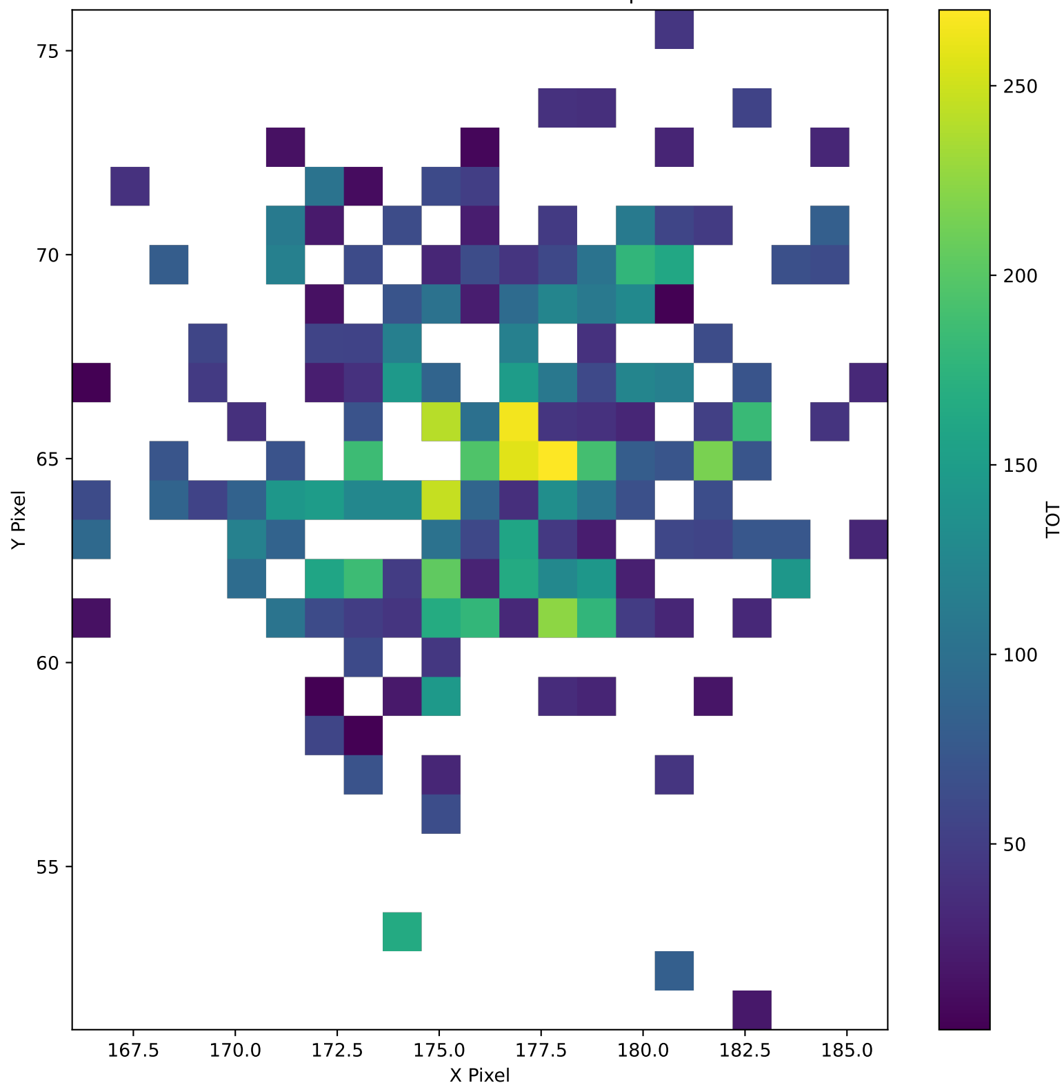
TrkID-2344173 TOT Pixel Map
