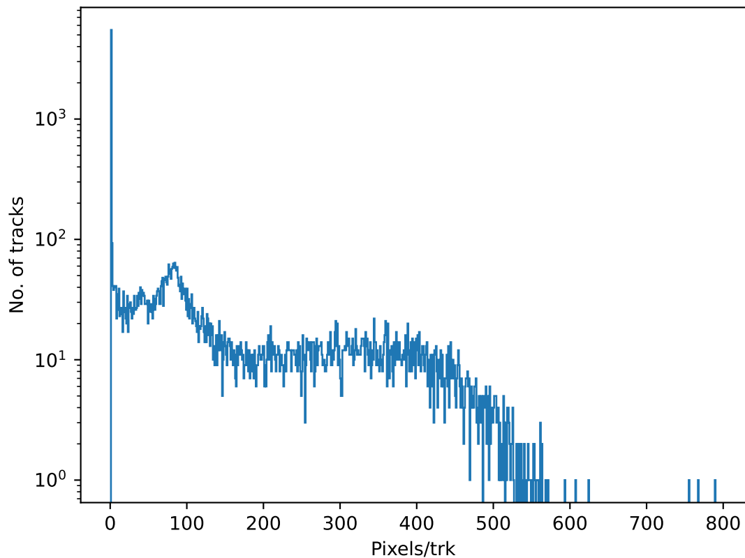
Trk Size (nrow) hist Ct rate : 112.38 sec-1
