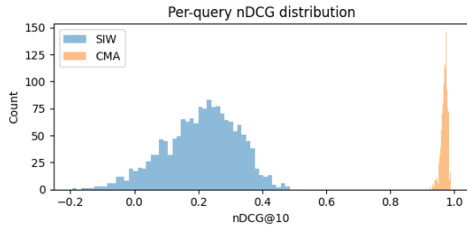
Fig. 2. Per-query nDCG histogram (CMA vs SIW).
