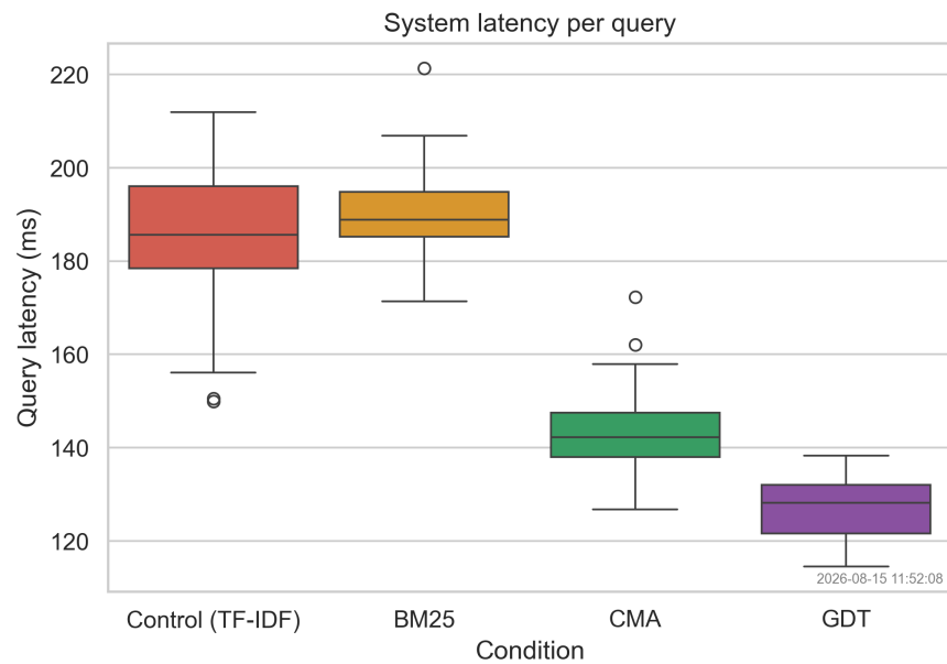
Figure 5: Query latency by condition (scale 10). GDT achieves the lowest latency (127.2 ms) versus Control (184.7 ms) and BM25 (190.0 ms).
