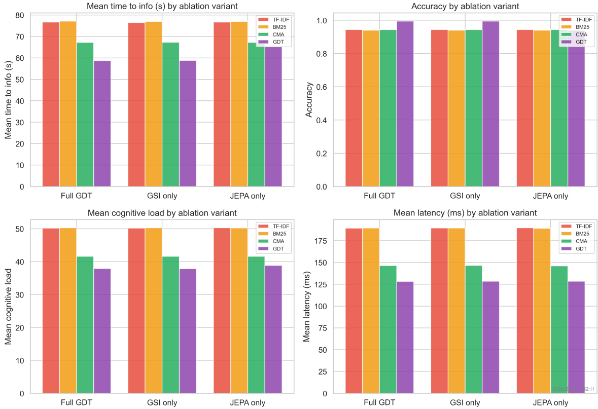
Figure 9: Four-arm component ablation at scale 1,000. Removing the GSI gate (JEPA-only) raises time-to-information and lowers completion; disabling prefetch (GSI-only) leaves metrics near Full GDT. GDT remains fastest and most accurate in every configuration.
