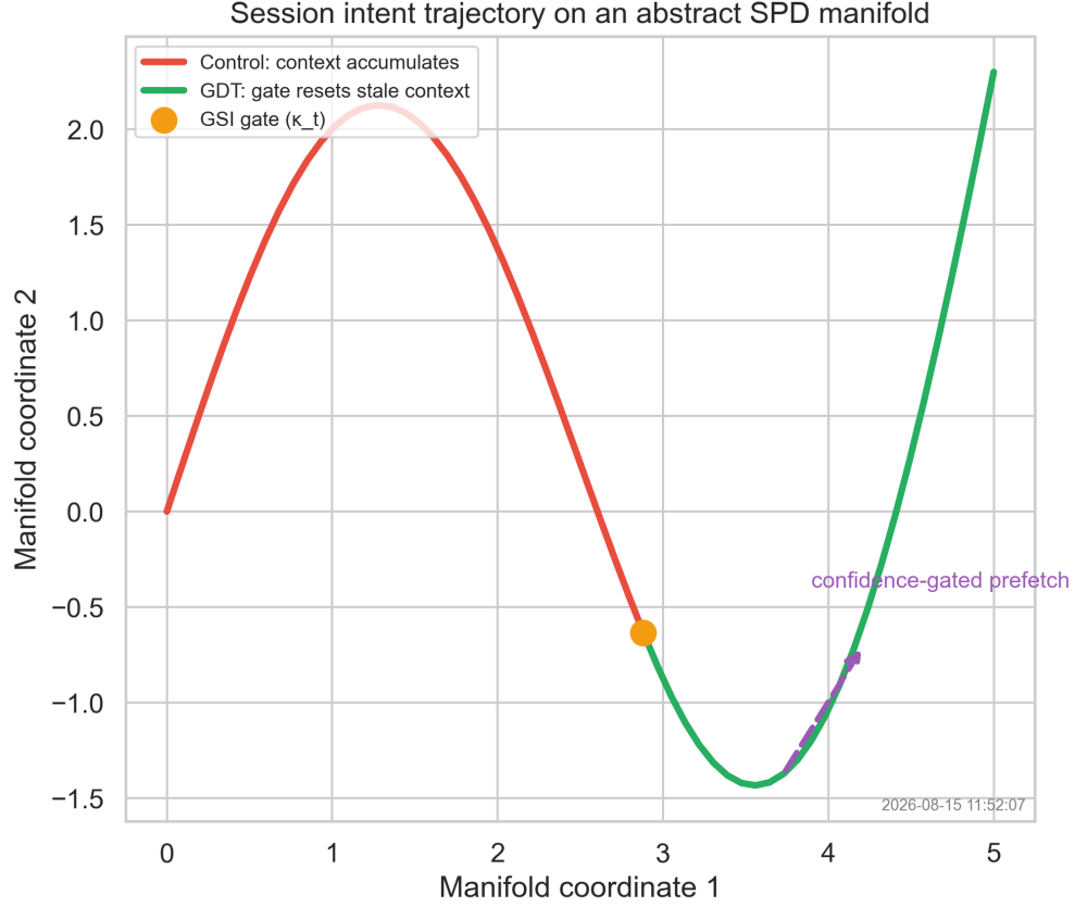
Figure 10: Geodesic intent trajectories on the SPD manifold \mathcal{S}_d^+ . The Control condition accumulates stale context across topic pivots; GDT with the Geodesic Shift Interference (GSI) gate suppresses stale context at large geodesic shifts, and the optimal-control prefetch engine forecasts next-intent embeddings. Larger benefit for multi-pivot tasks confirms the mechanism.
