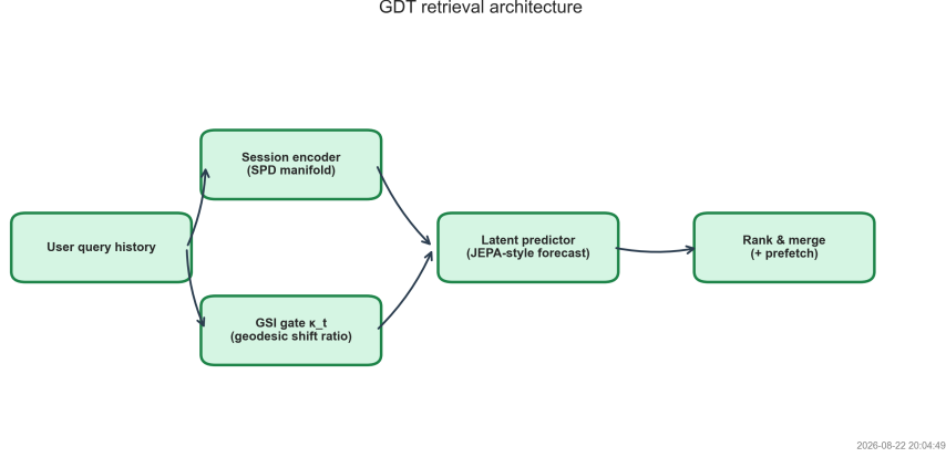
Figure 11: Geodesic Diagnostic Trajectories (GDT) component overview (representative scale). component behavior and layout are consistent across scales.
