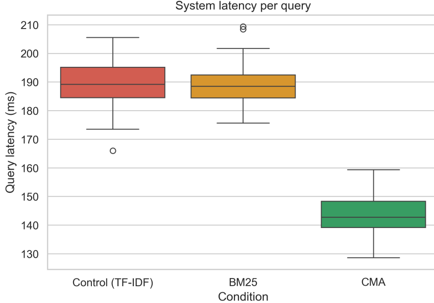
Figure 2: Mean retrieval latency per query. CMA achieved a 23.8% reduction (144.0 ms vs 189.0 ms, p < 0.001 , d = -3.91 ) via JEPA-driven prefetching; the TF-IDF and BM25 baselines were indistinguishable.
