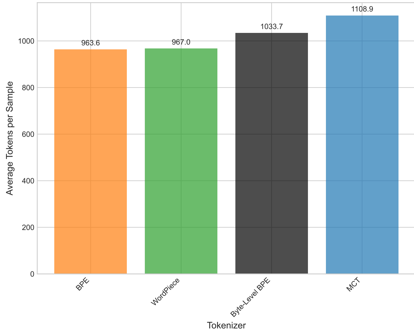
Tokenization Compactness
