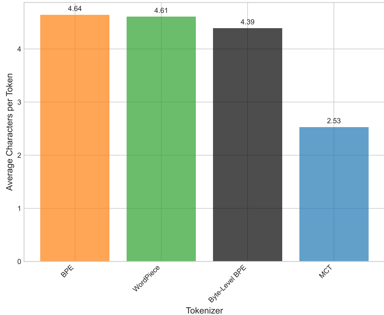
Tokenization Efficiency
