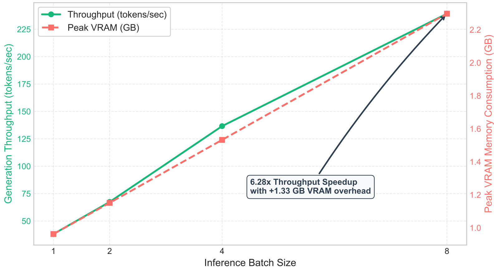
Inference Latency/Throughput Scaling & Peak VRAM footprint
