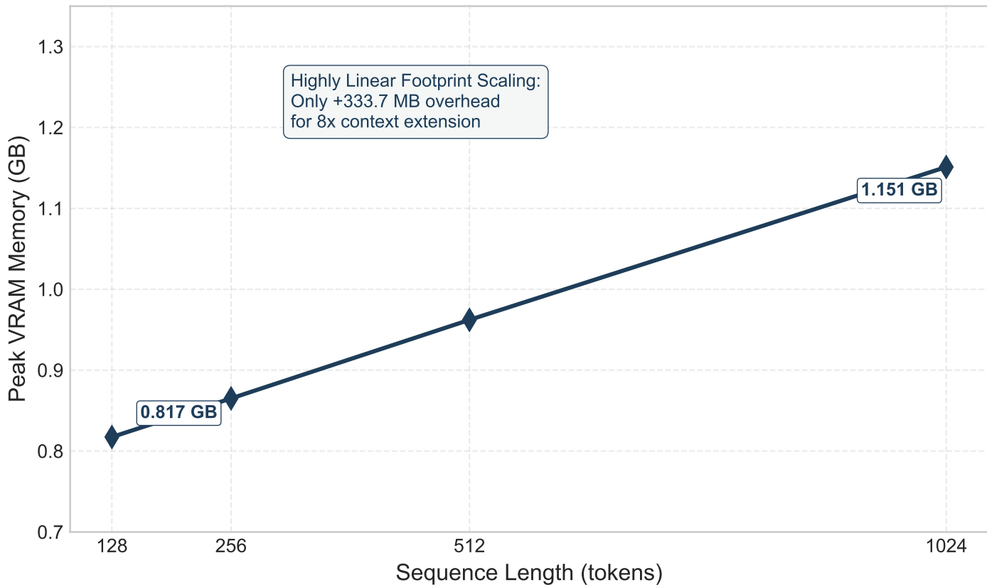
Inference Peak VRAM Footprint vs. Context Sequence Length
