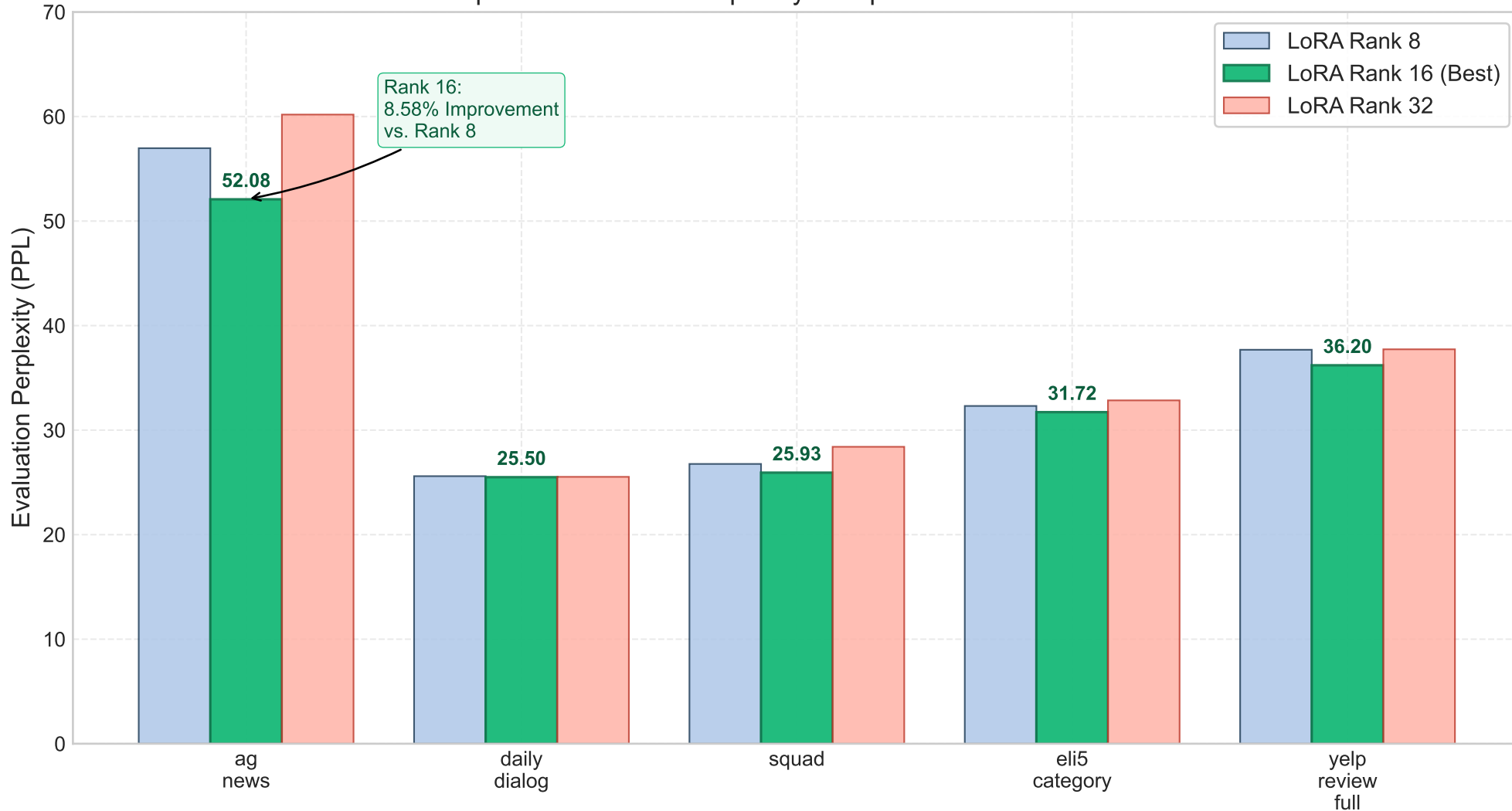
Step 2000 Validation Perplexity Comparison Across Domains
