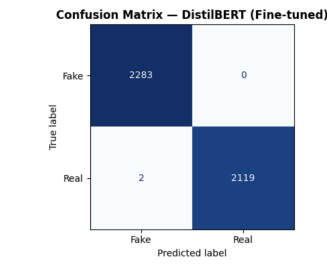
Fig. 3. Confusion matrix for fine-tuned DistilBERT showing only 2 misclassifications out of 4,404 test articles.
