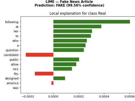
Fig. 6. LIME explanation for a fake news article (99.56% confidence). Red bars push toward Fake, green bars toward Real.
