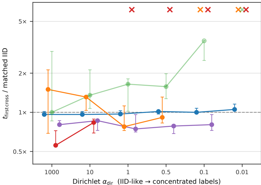
Time to Generalise under Label Skew ( K = 10 )
