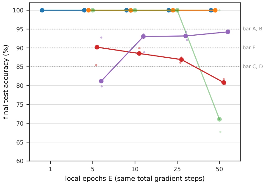
Final Test Accuracy vs Local Epochs (K = 10)
