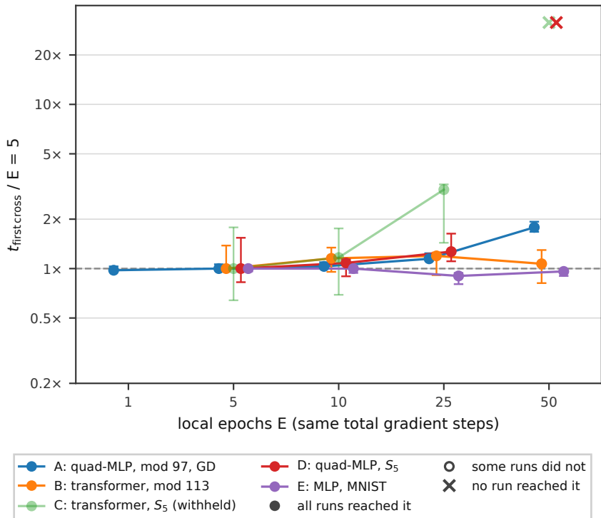
Time to Generalise vs Local Epochs ( K = 10 )
