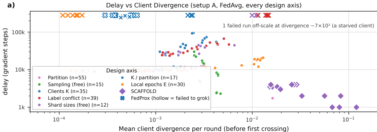
Delay vs Client Divergence (setup A, FedAvg, every design axis)
