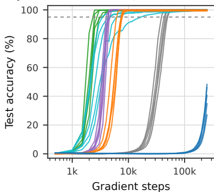
b) H1: \alpha=0.25 , E=25, IID
