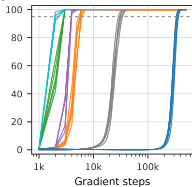
d) H3: \alpha=0.3 , E=50, non-IID
