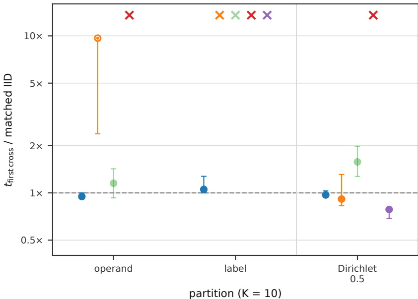
Time to Generalise by Partition
