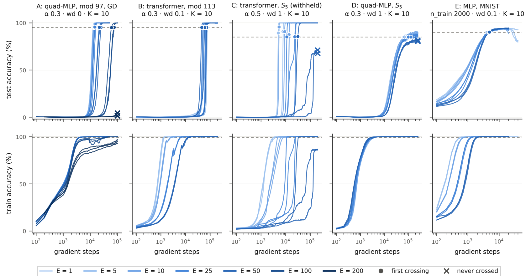
Training Curves per Run across Local Epochs (same total gradient steps)
