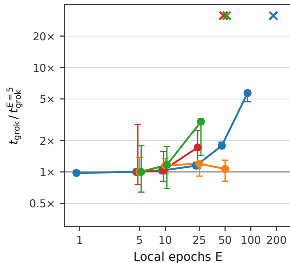
b) Time to Generalise vs Local Epochs
