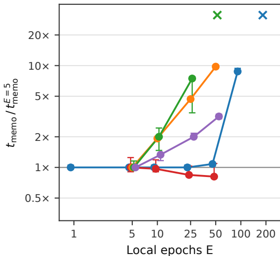
a) Time to Memorise vs Local Epochs
