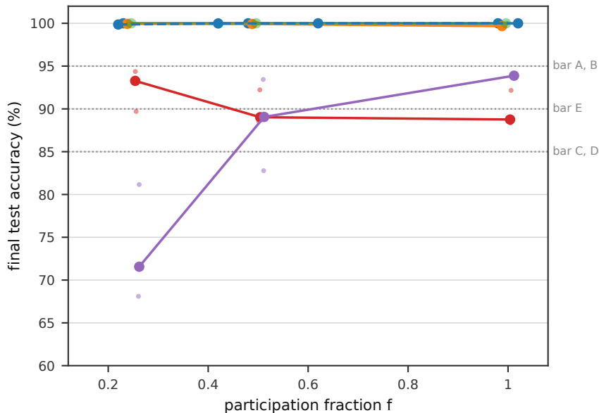
Final Test Accuracy vs Participation
