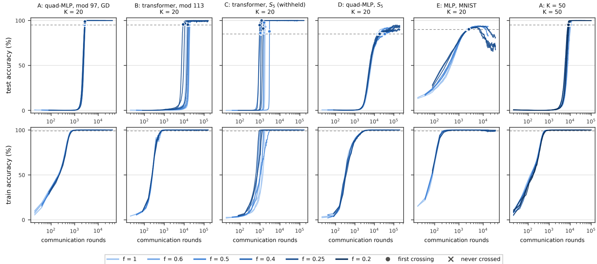
Training Curves per Run across Participation Fractions (x = rounds)
