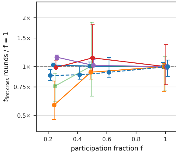
b) Rounds to Generalise vs Participation
