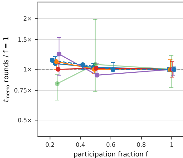
a) Rounds to Memorise vs Participation
