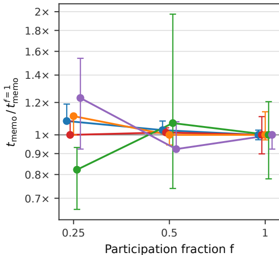
a) Rounds to Memorise vs Participation
