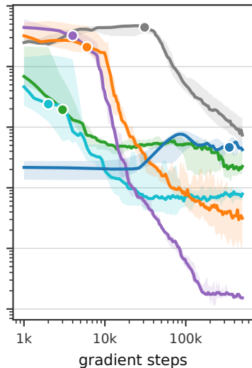
Client Divergence over Training by Aggregation Rule (setup A, K = 10 ) median over 5 seeds, smoothed; band = range over seeds
