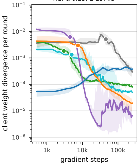
Client Divergence over Training by Aggregation Rule (setup A, K = 10 ) median over 5 seeds, smoothed; band = range over seeds
