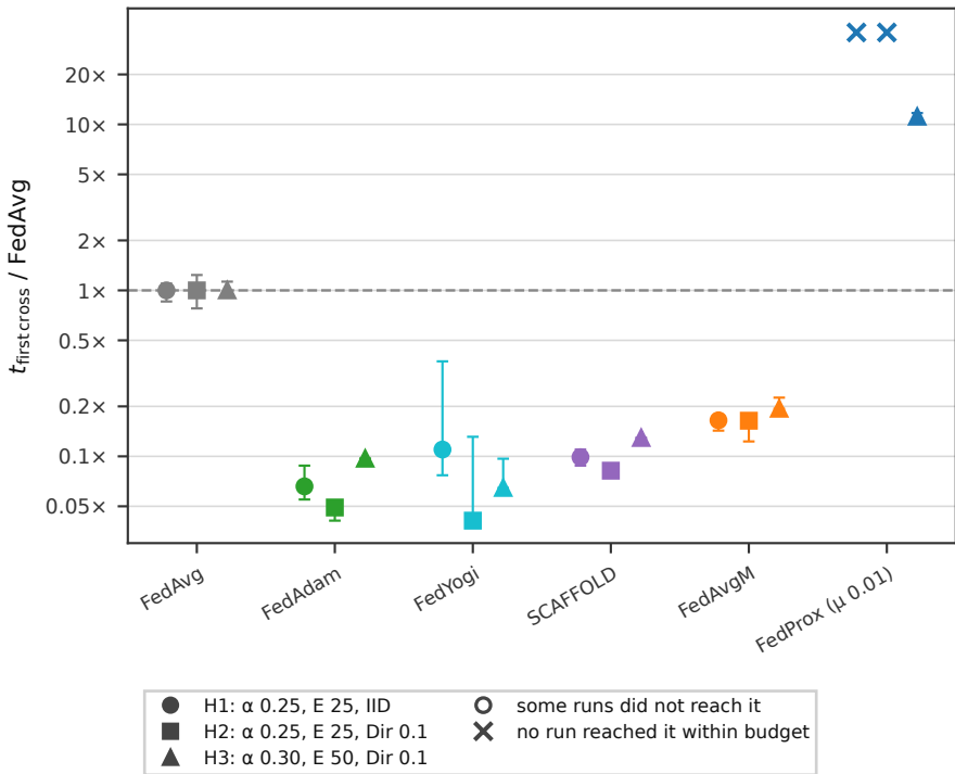
Time to Generalise by Aggregation Rule (A, K = 10)
