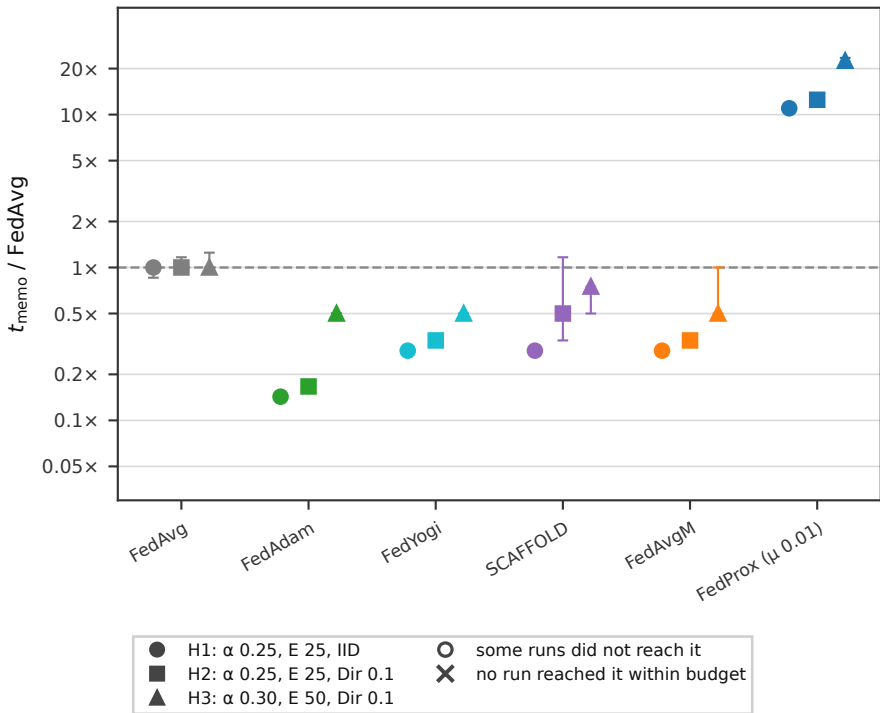
Time to Memorise by Aggregation Rule (A, K = 10)
